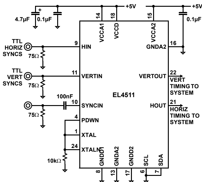
FIGURE 8. APPLICATIONS DRAWING 1
