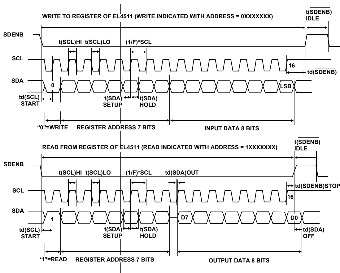
FIGURE 11. SERIAL INTERFACE TIMING DIAGRAM
