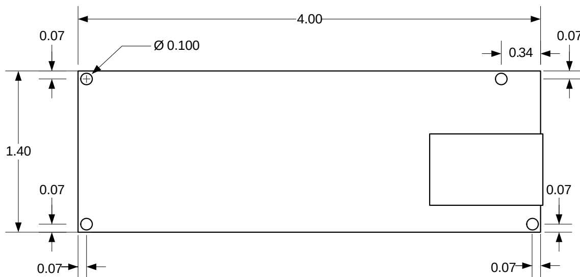
Figure B-3. EK-LM3S9B92 Evaluation Board Dimensions
