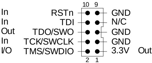
Figure 2-3. JTAG/SWD Connector
