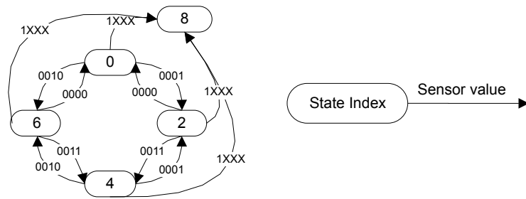
Figure 28.19. FSM Example 2
