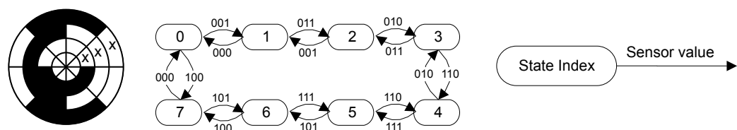
Figure 28.18. FSM Example 1
