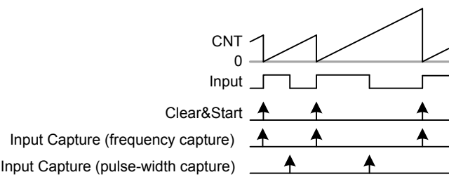
Figure 20.13. TIMER/WTIMER Period and/or Pulse width Capture
