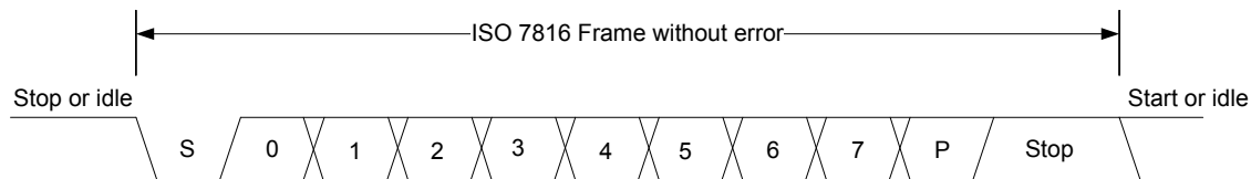
Figure 18.14. USART ISO 7816 Data Frame Without Error
