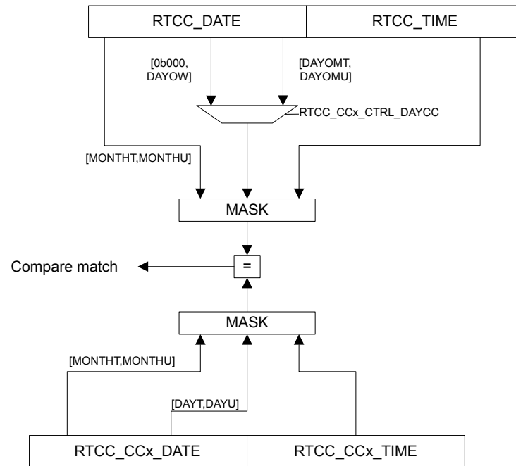
Figure 13.5. RTCC Compare in calendar mode, COMPBASE = CNT
