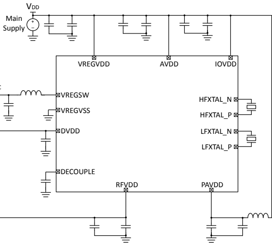
Figure 5.3. EFR32BG1 Typical Application Circuit: Configuration with DC-DC converter (PAVDD from VDD)
