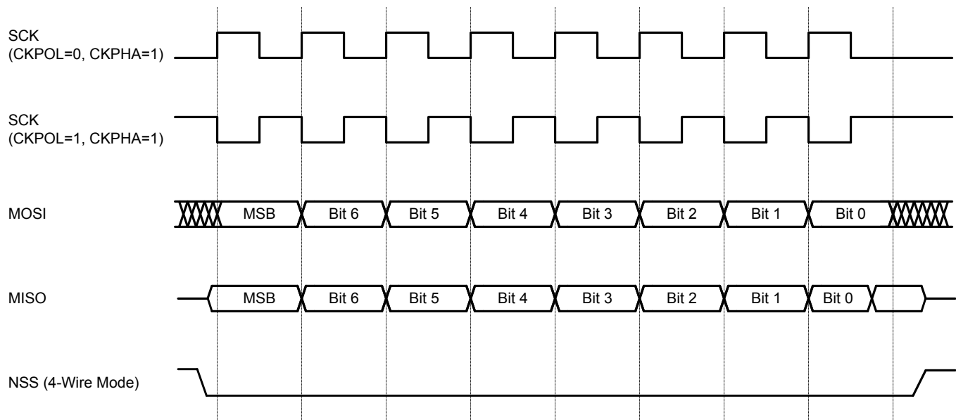
Figure 16.7. Slave Mode Data/Clock Timing (CKPHA = 1)
