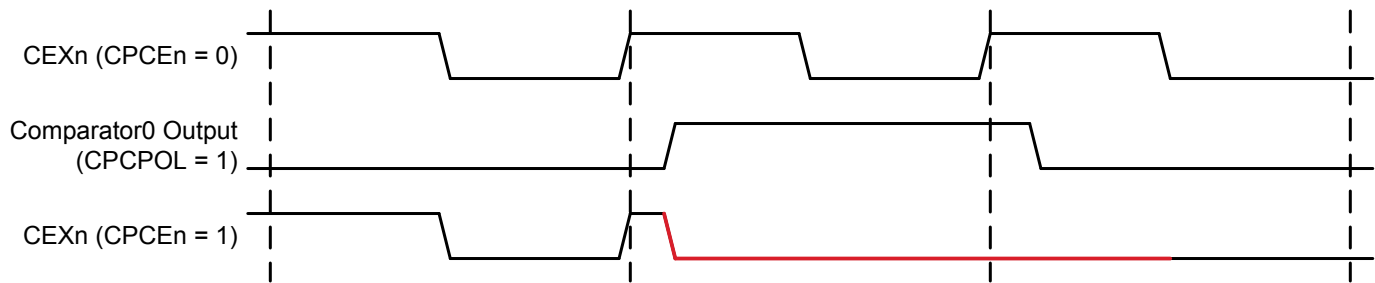
Figure 15.15. CEXn with CPCEn = 1, CPCPOL = 1
