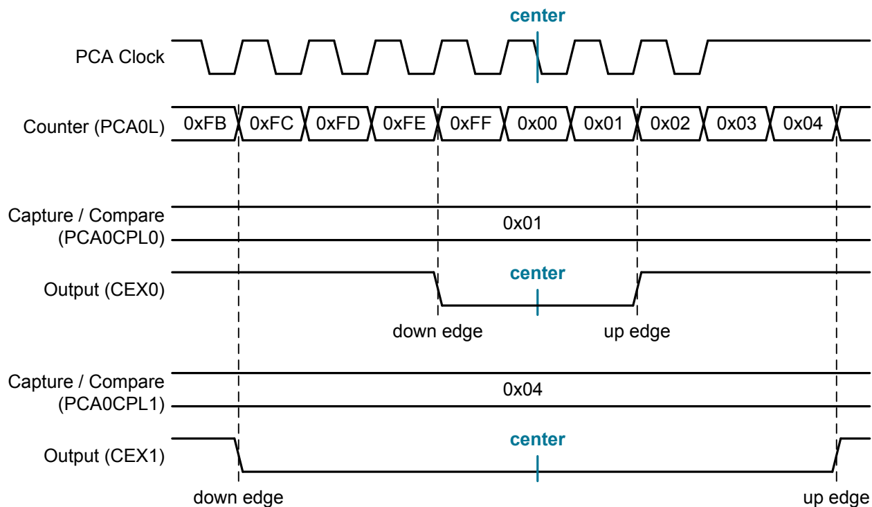
Figure 15.9. Center-Aligned PWM Timing
