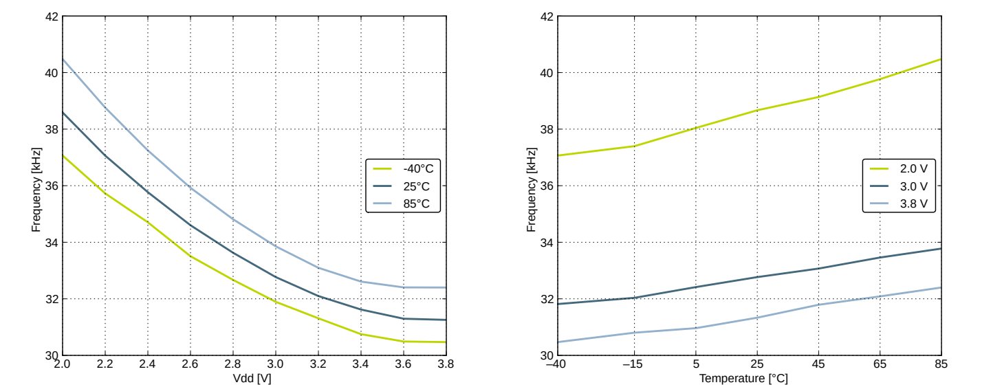
Figure 4.10. Calibrated LFRCO Frequency vs Temperature and Supply Voltage
