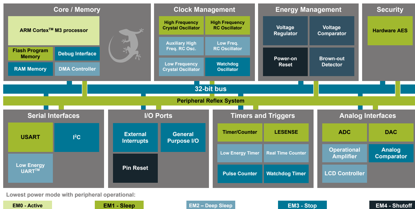
Figure 3.1. Block Diagram
