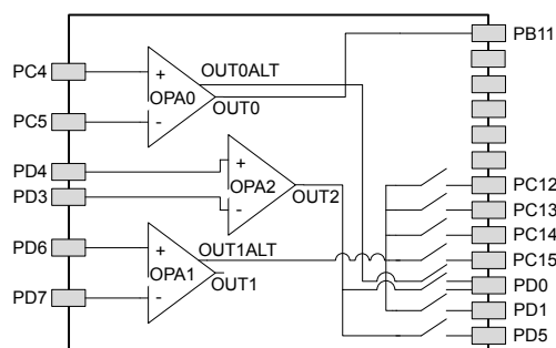
Figure 5.21. Opamp Pinout
