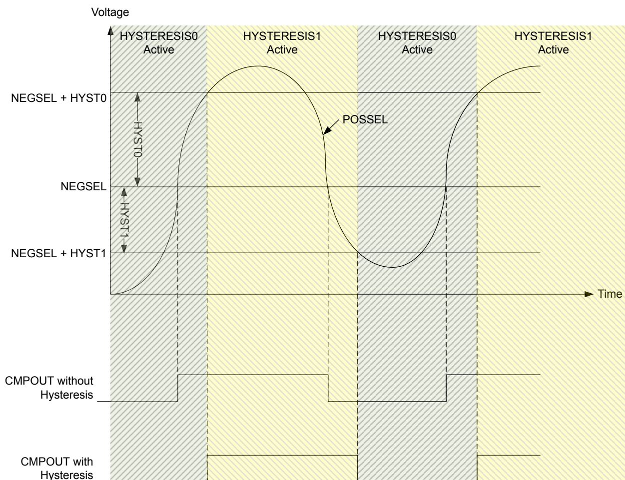
Figure 21.3. Hysteresis
