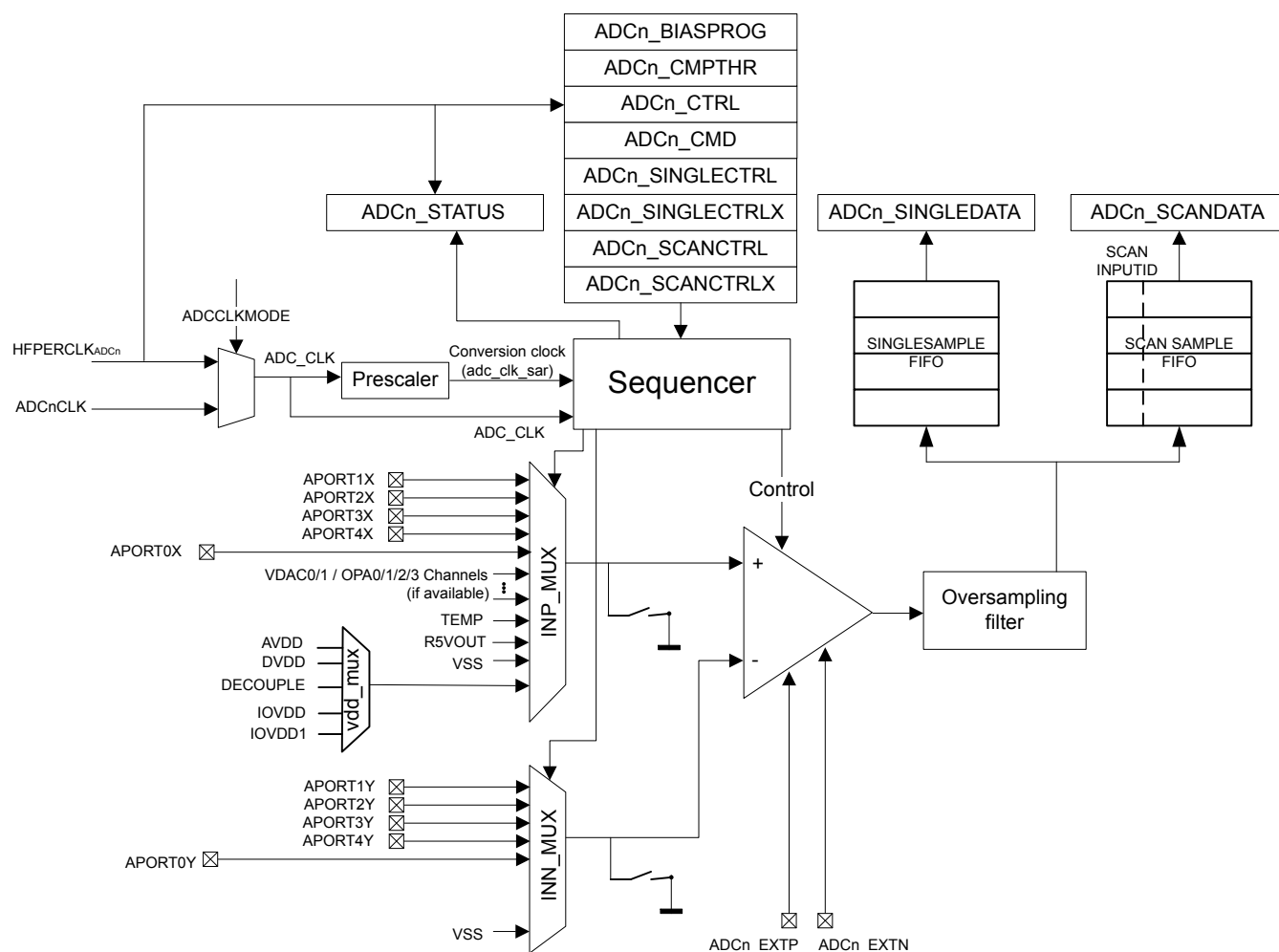
Figure 22.1. ADC Overview
