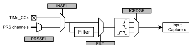
Figure 18.11. TIMER Input Pin Logic
