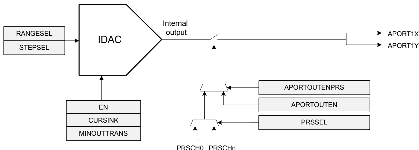
Figure 23.1. IDAC Overview
