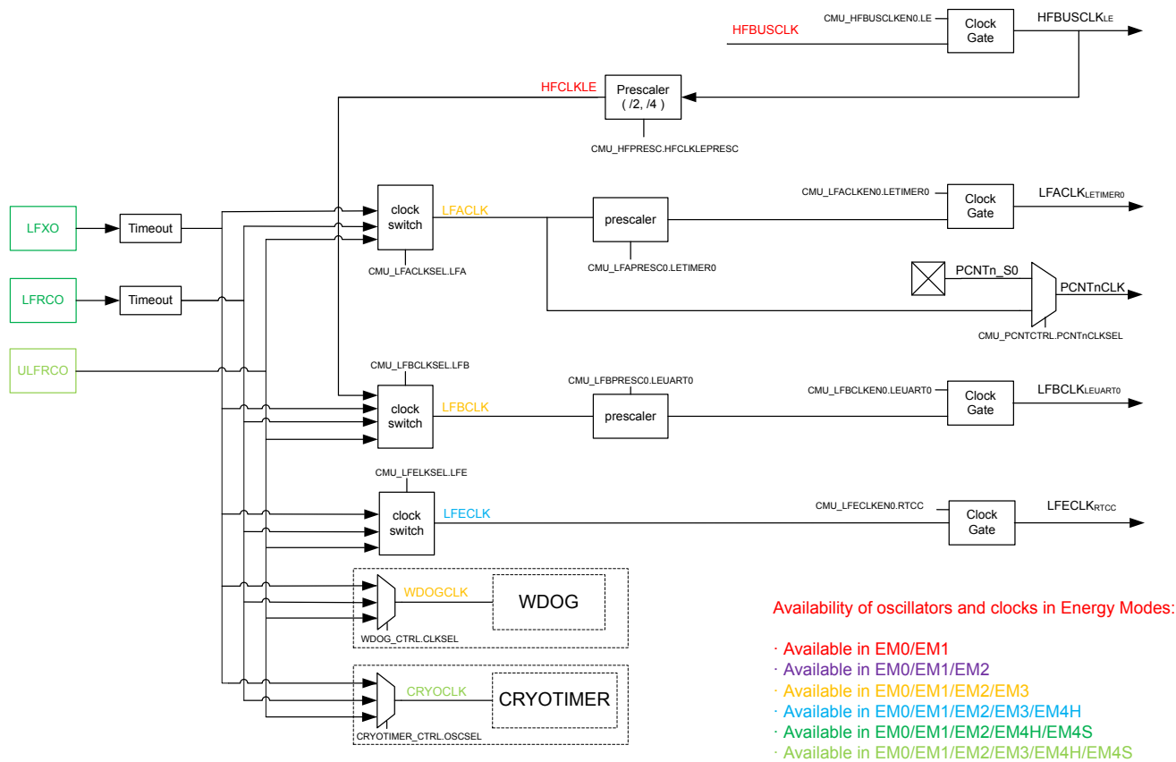
Figure 10.2. CMU Overview - Low Frequency Portion
