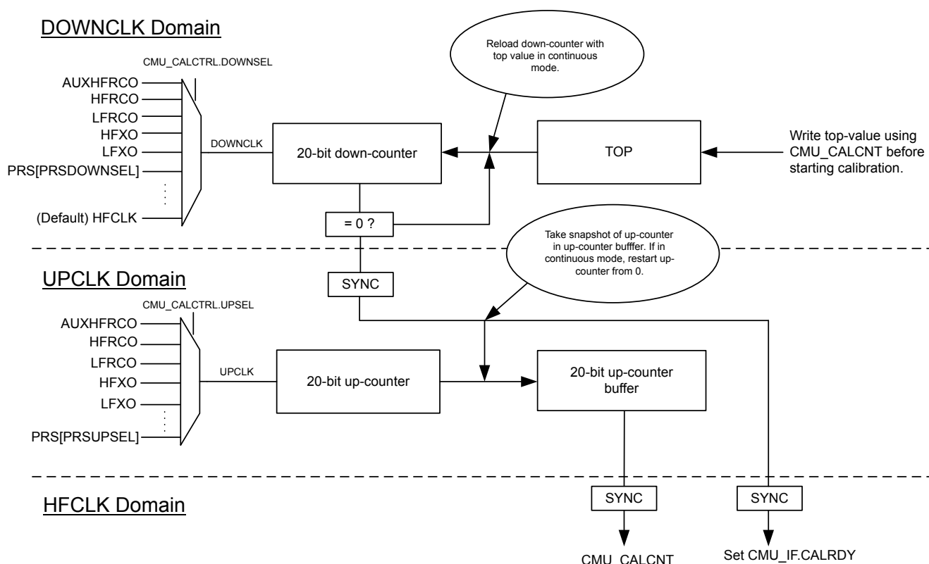
Figure 10.12. HW-support for RC Oscillator Calibration
