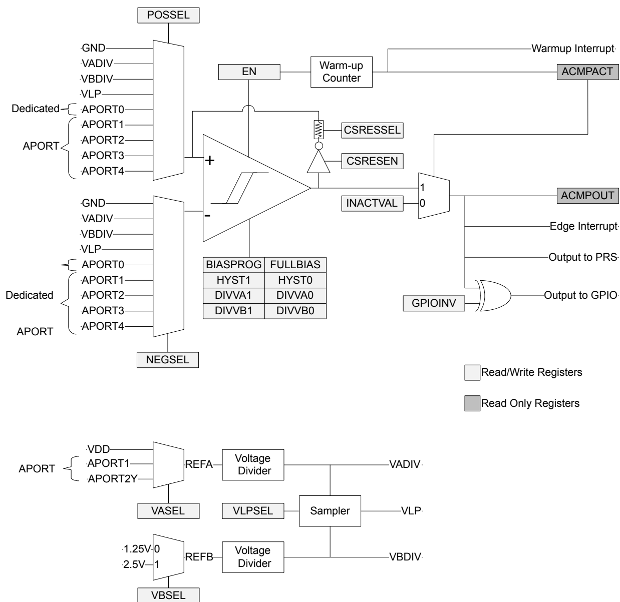
Figure 21.1. ACMP Overview
