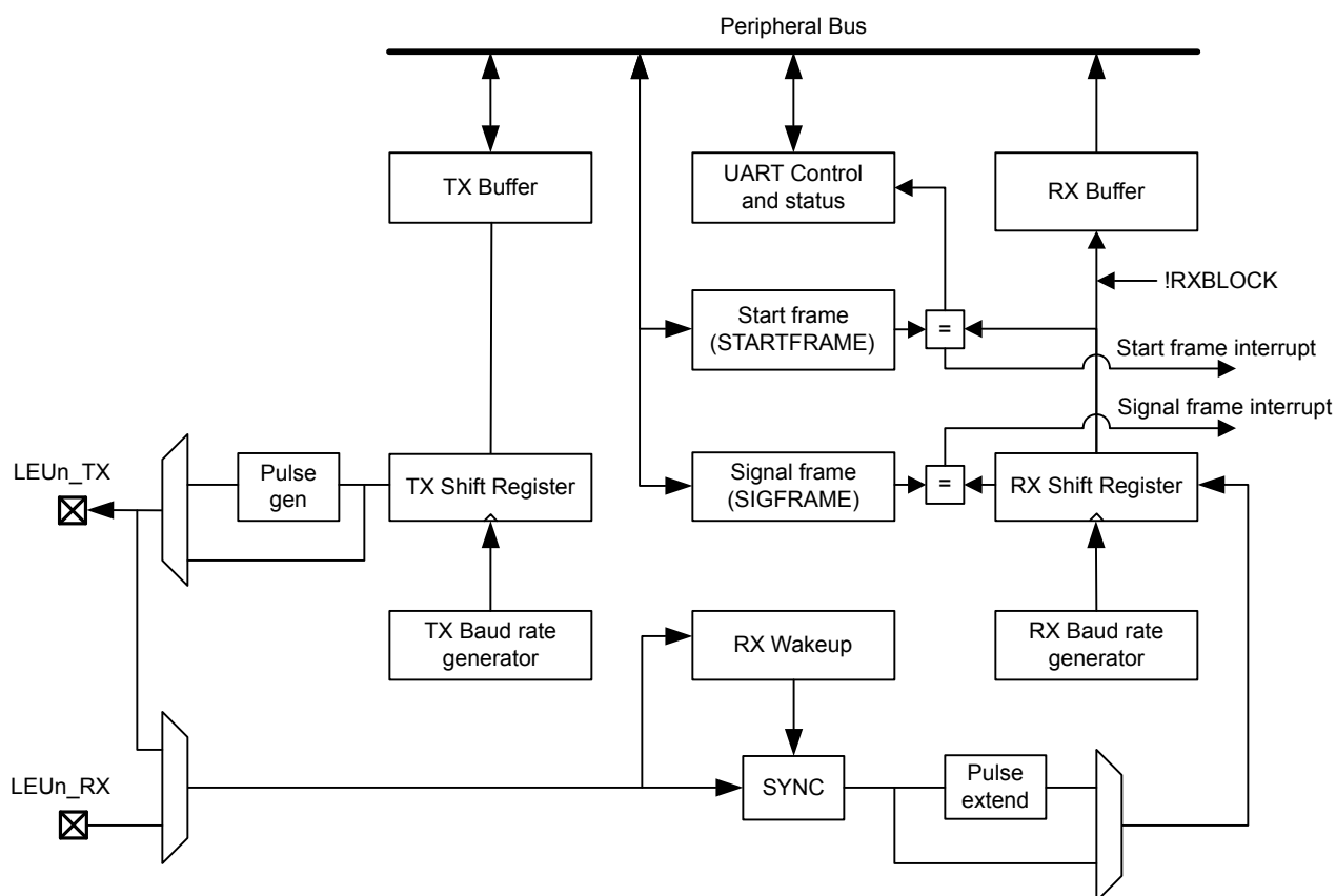
Figure 17.1. LEUART Overview
