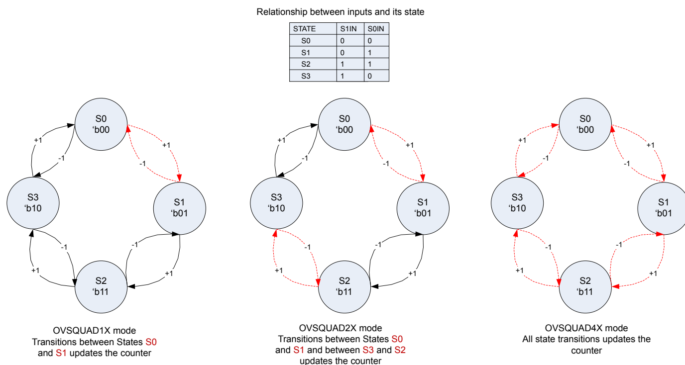
Figure 14.3. PCNT State Transitions for Different Oversampling Quadrature Decoder Modes
