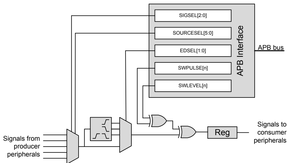
Figure 13.1. PRS Overview
