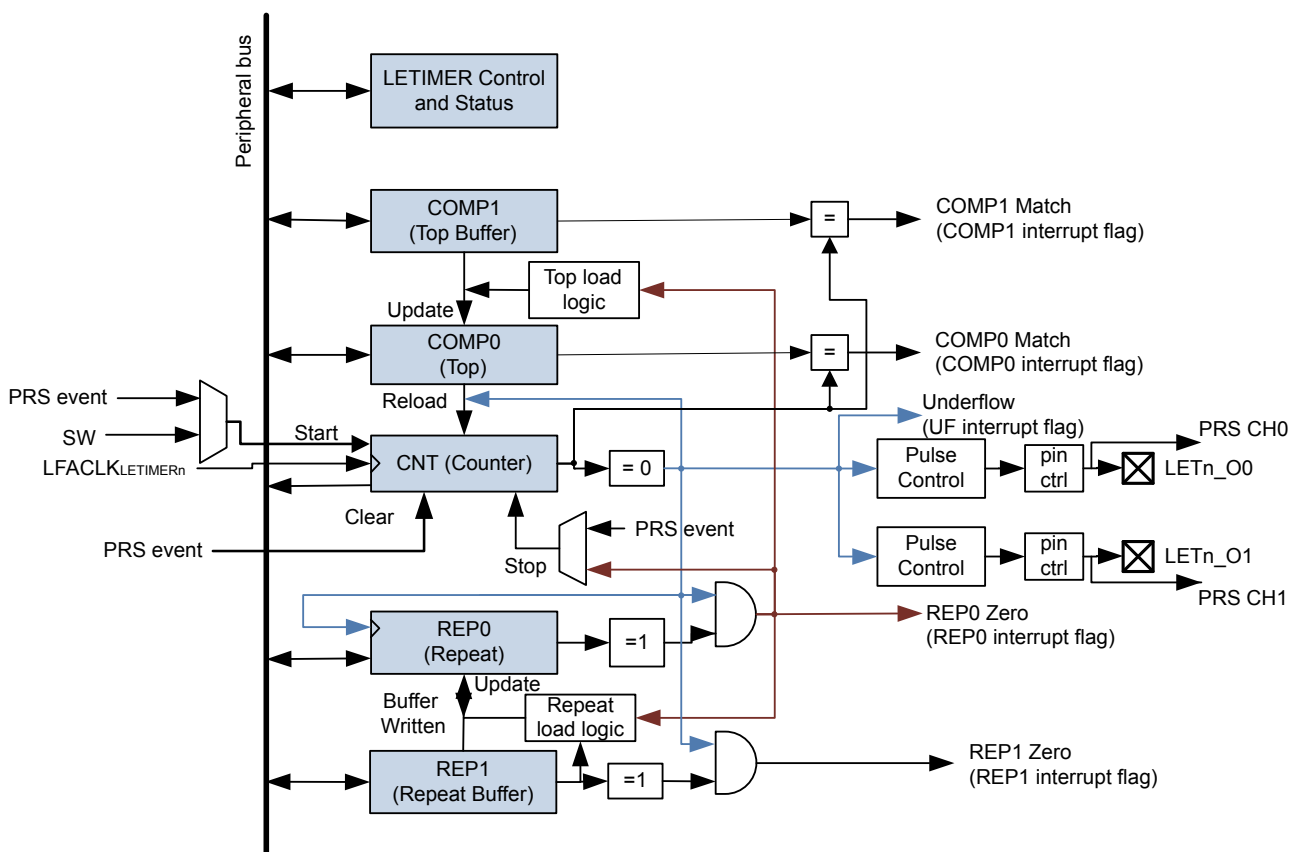
Figure 19.1. LETIMER Overview
