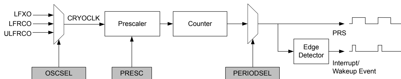
Figure 20.1. CRYOTIMER Block Overview
