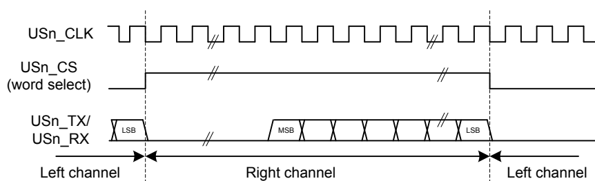
Figure 16.23. USART Right-Justified I2S Waveform
