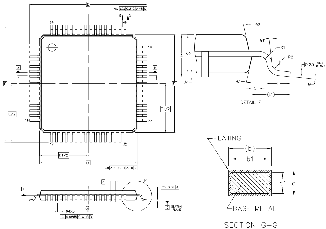
Figure 9.1. TQFP64
