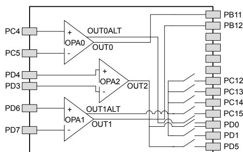
Figure 5.34. Opamp Pinout
