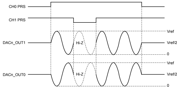
Figure 24.6. VDAC Sine Mode
