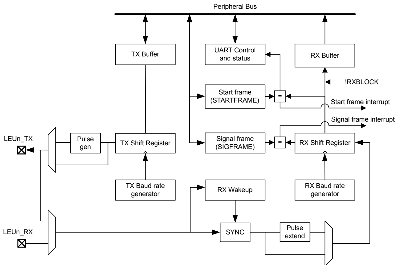
Figure 20.1. LEUART Overview
