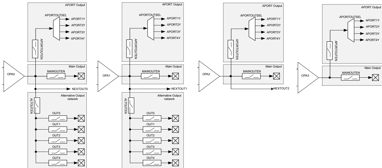
Figure 25.3. Opamp Output Stage Overview
