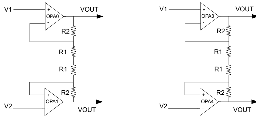
Figure 25.11. Instrumentaion Amplifier Overview
