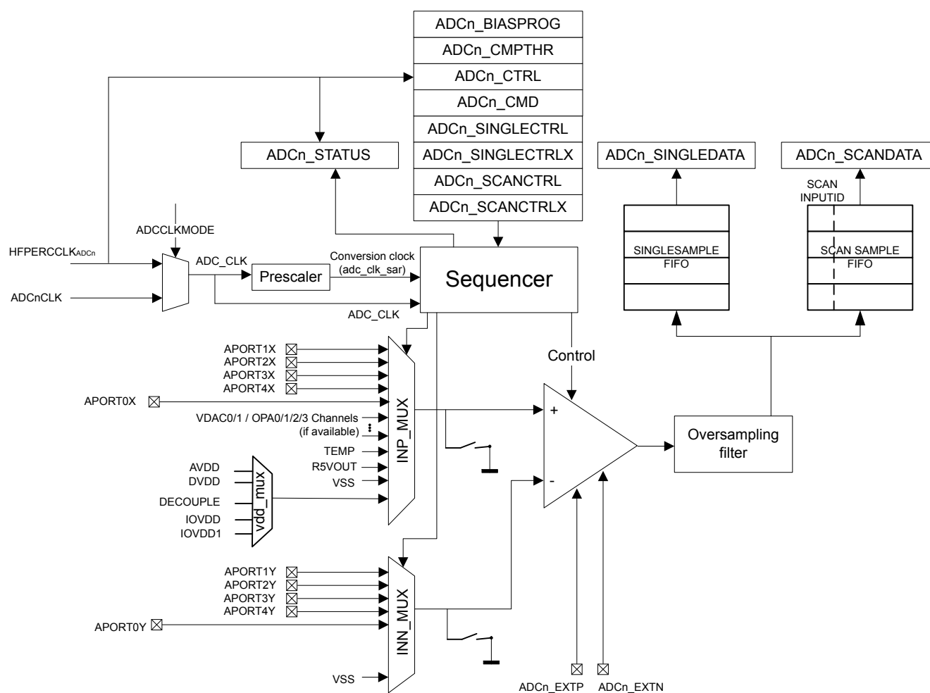
Figure 27.1. ADC Overview
