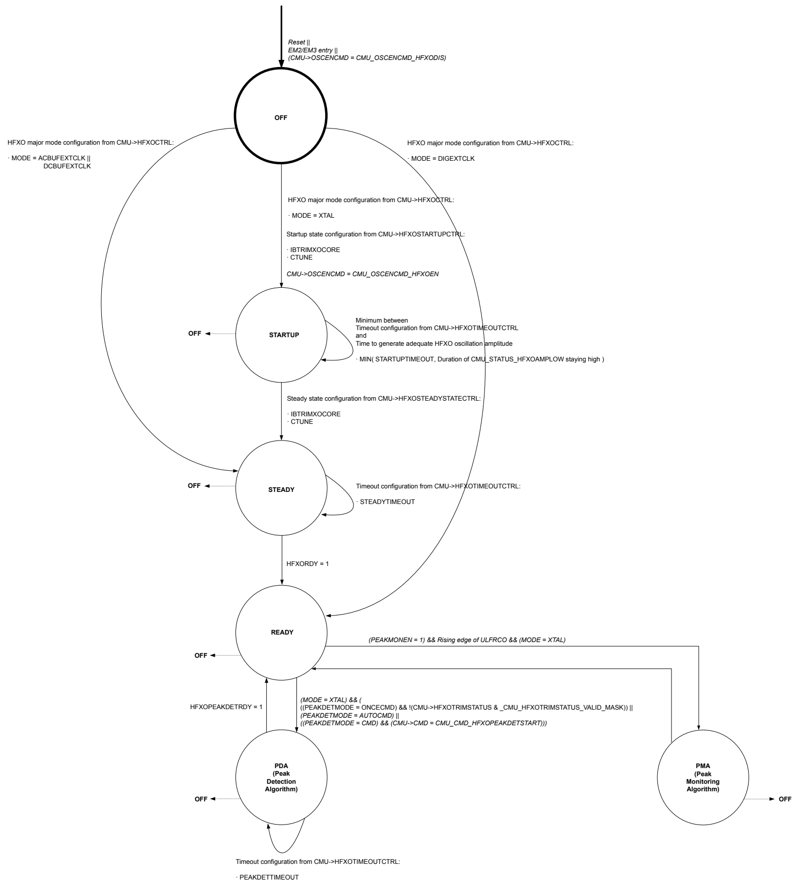
Figure 10.7. CMU HFXO control state machine
