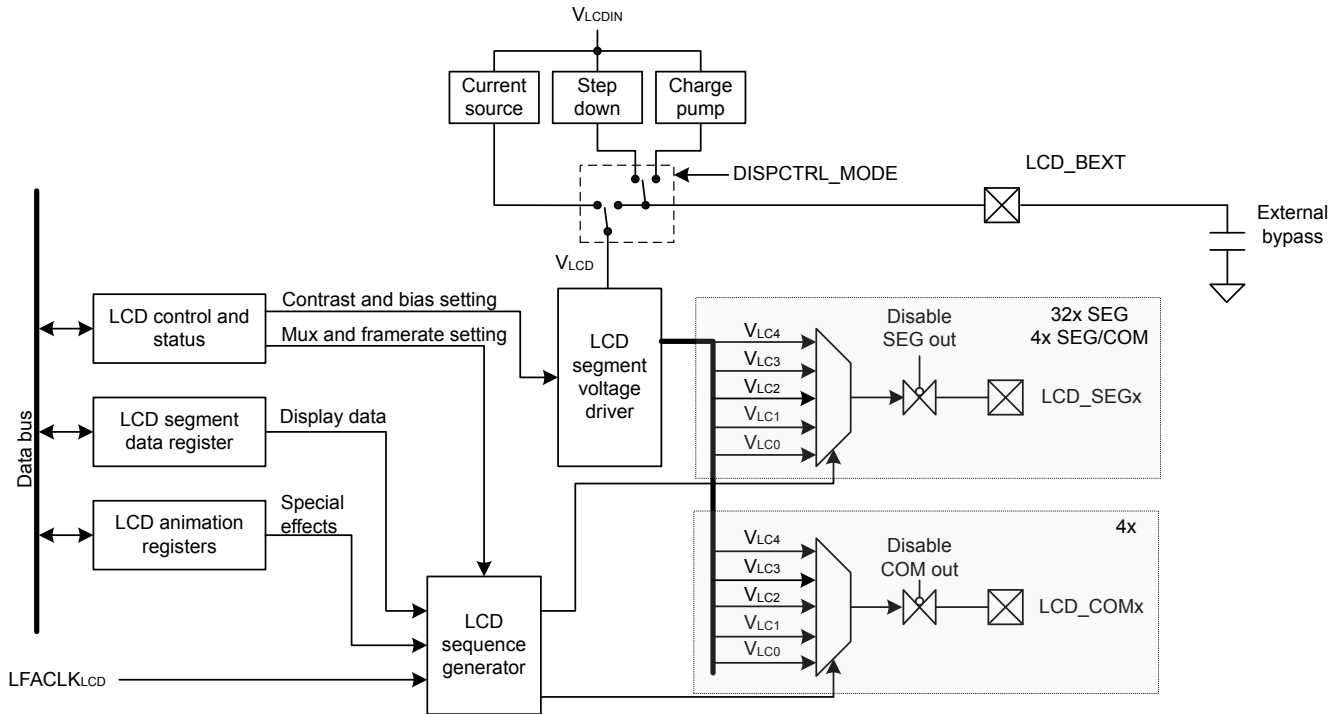
Figure 15.1. LCD Block Diagram
