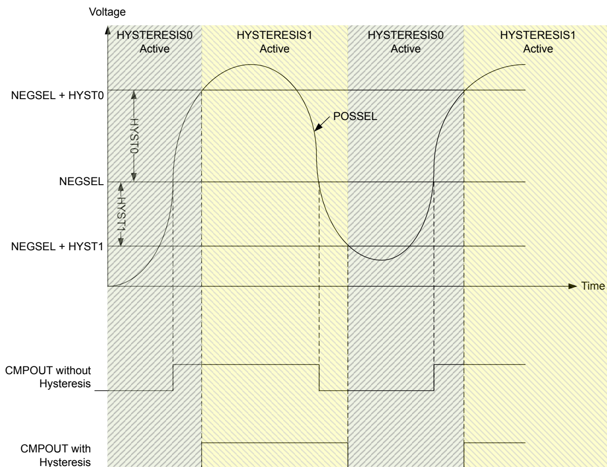
Figure 27.3. Hysteresis
