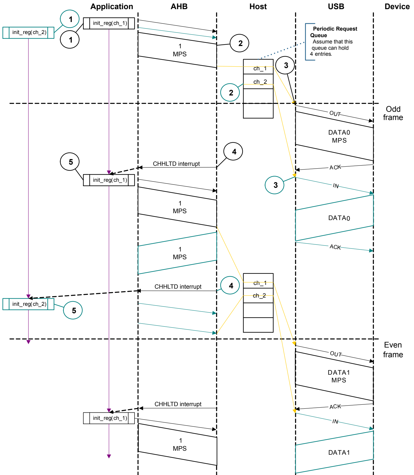
Figure 38.14. Normal Interrupt OUT/IN Transactions in DMA Mode
