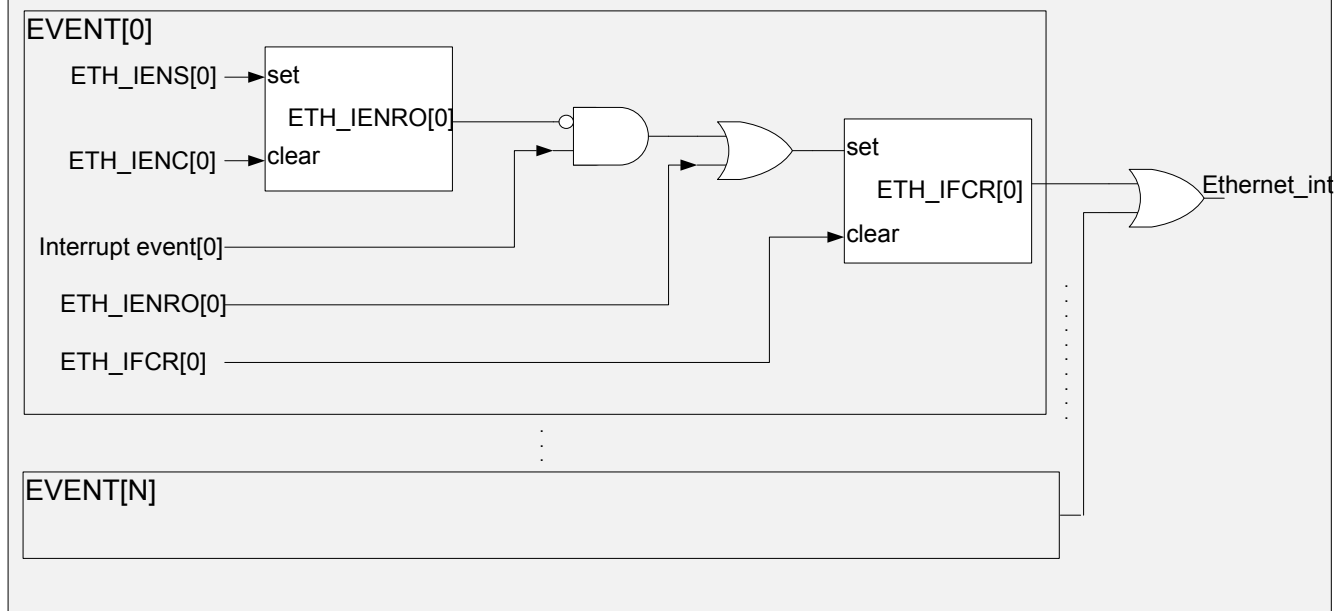
Figure 40.9. ETH Interrupt generation
