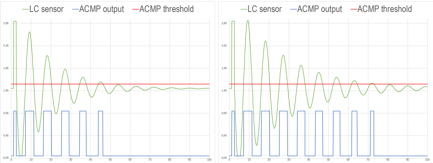
Figure 30.17. LC Sensor Oscillations
