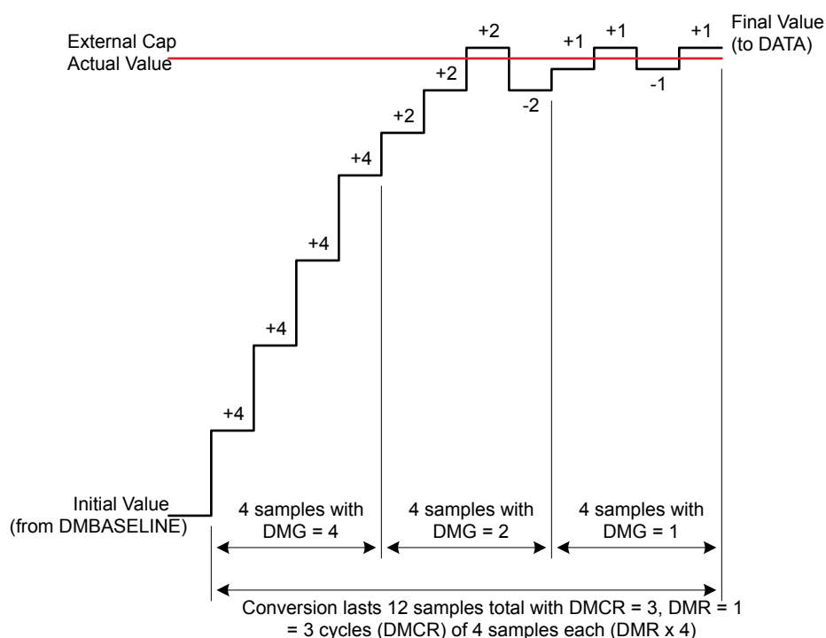
Figure 41.2. Delta Modulation Conversion With Gain Reduction (DMCFG_DMGRDIS = 0)
