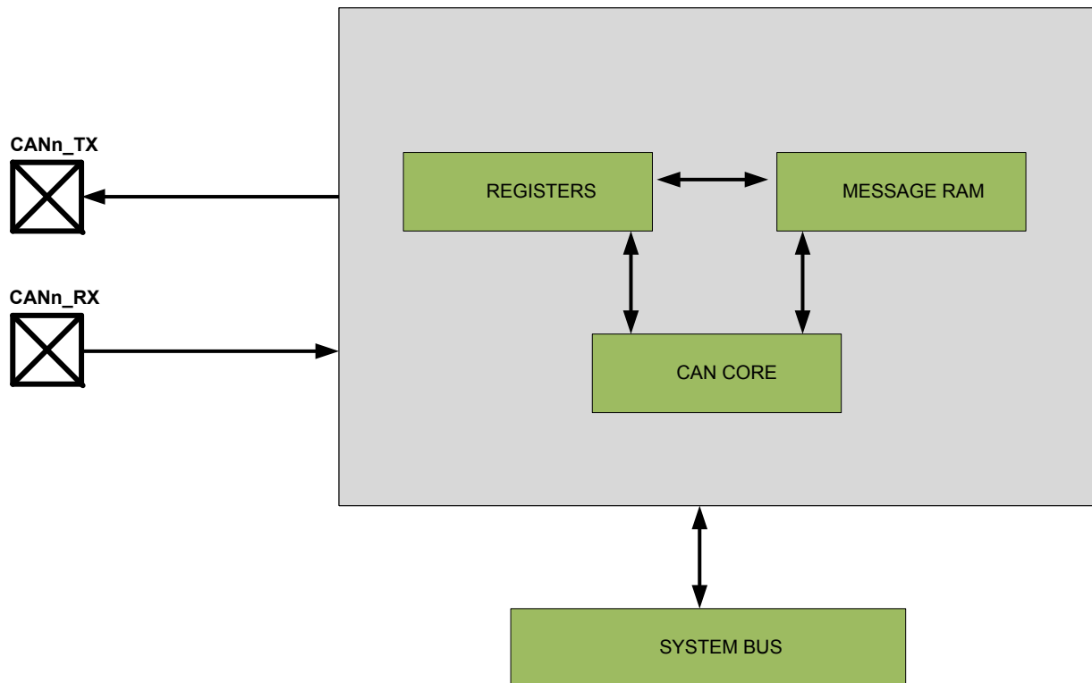
Figure 42.1. Block Diagram
