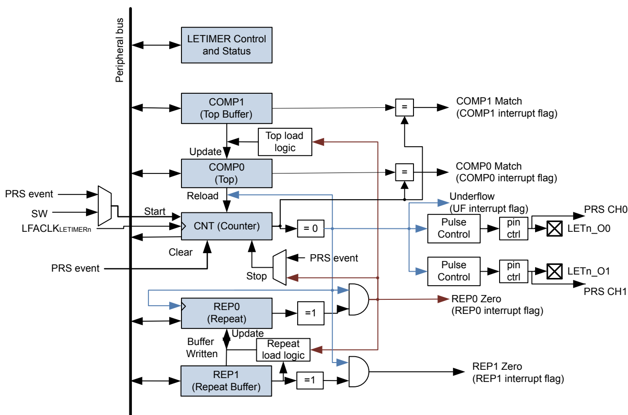
Figure 23.1. LETIMER Overview
