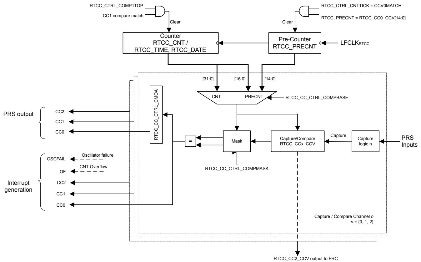
Figure 12.1. RTCC Overview
