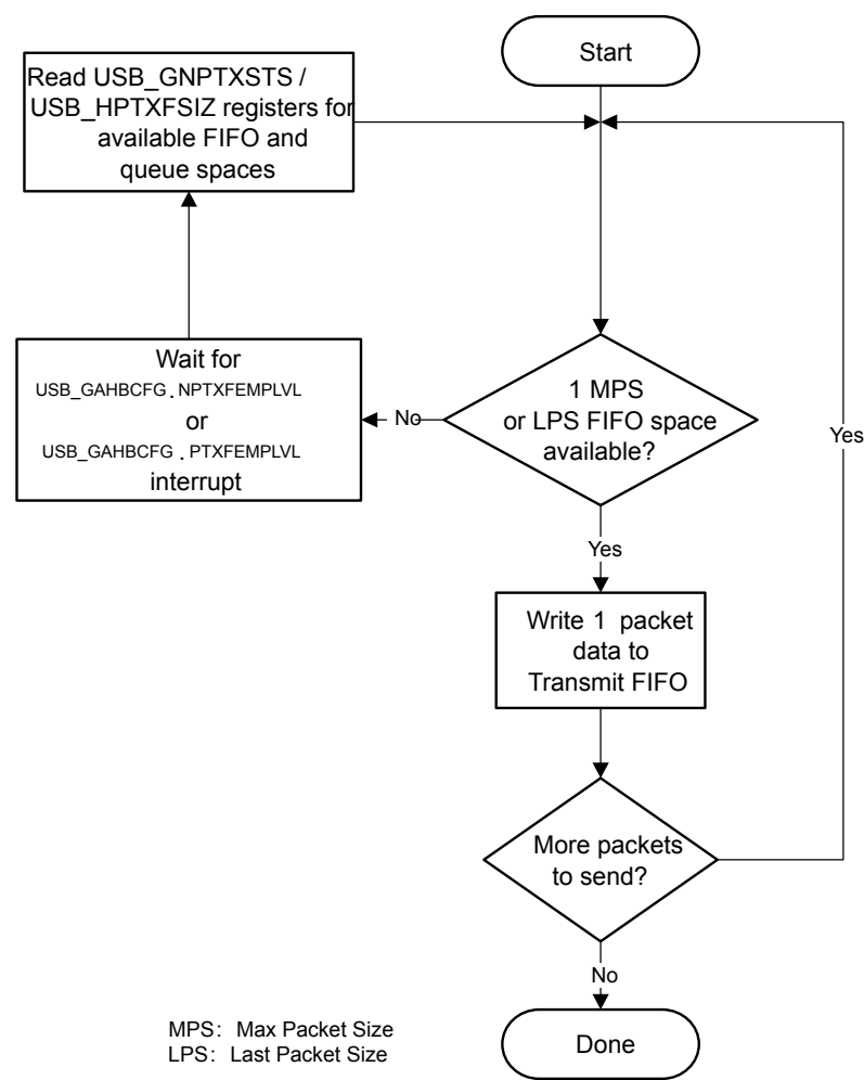
Figure 38.8. Transmit FIFO Write Task in Slave Mode
