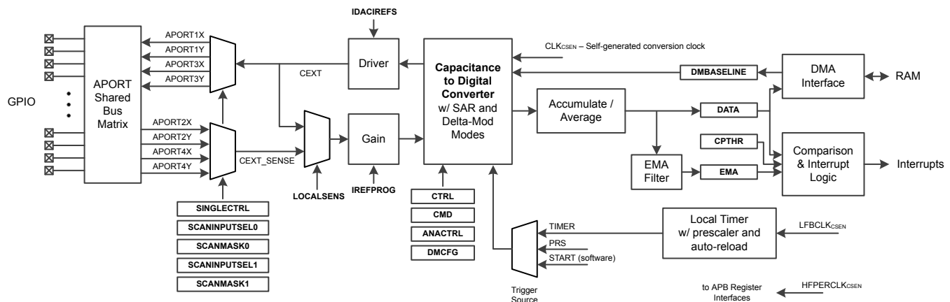
Figure 41.1. CSEN Overview
