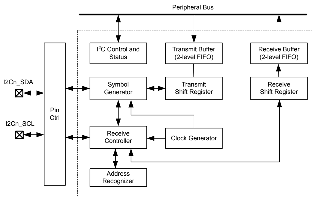
Figure 18.1. I2C Overview
