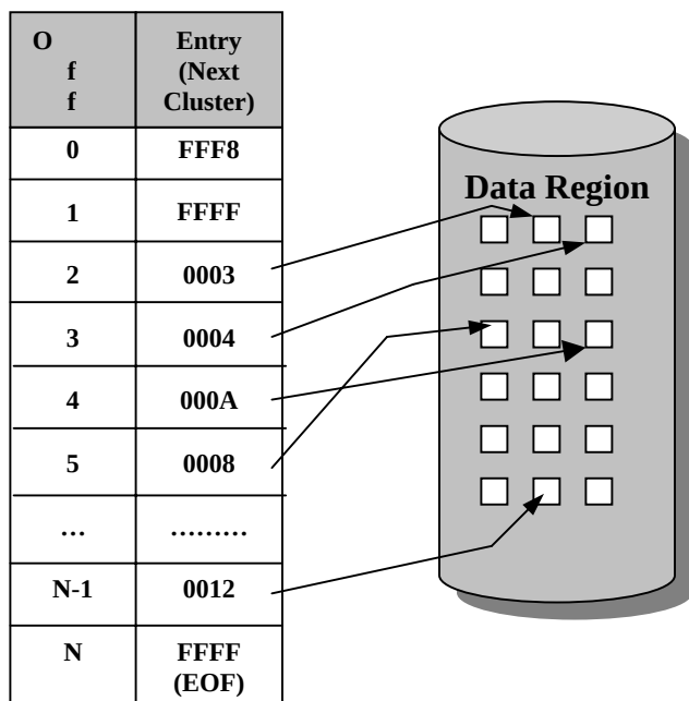
Figure 4. FAT File System
