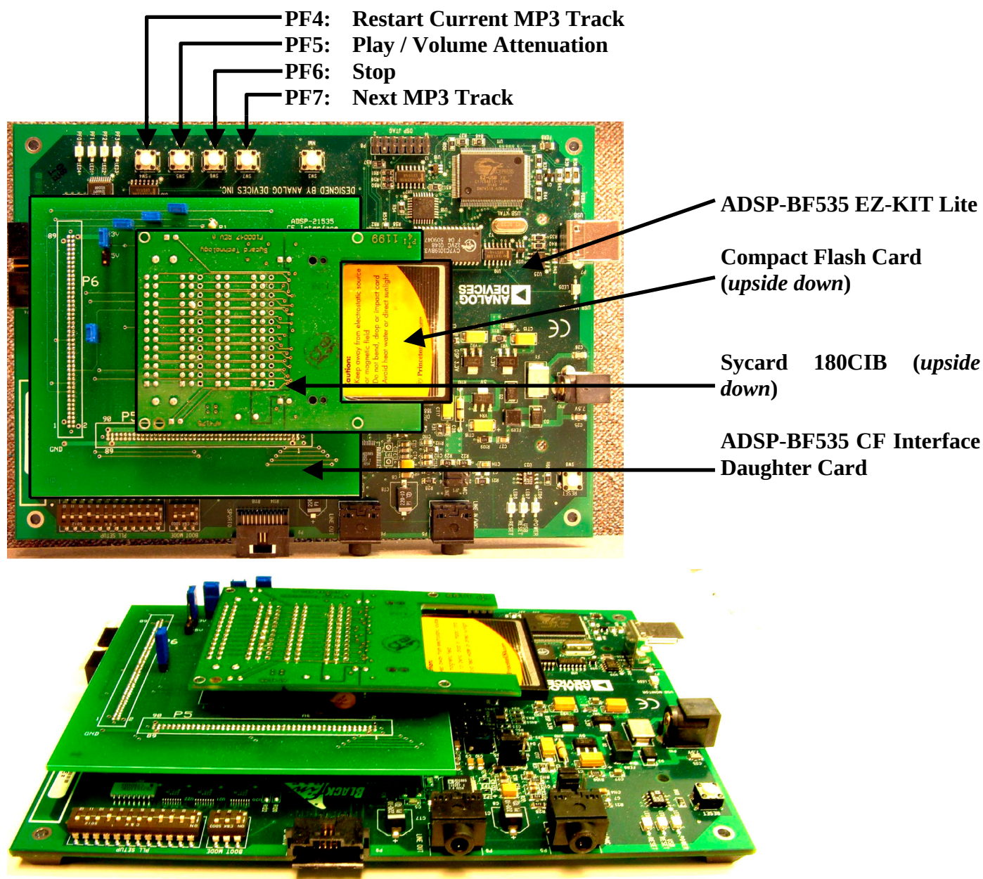
Figure 10. ADSP-BF535 CompactFlash Interface
