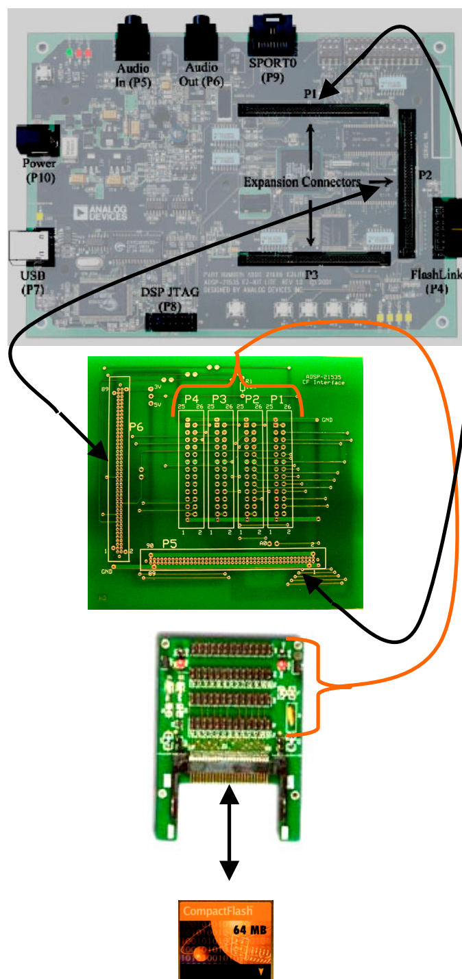
Figure 9. Physical Connections
