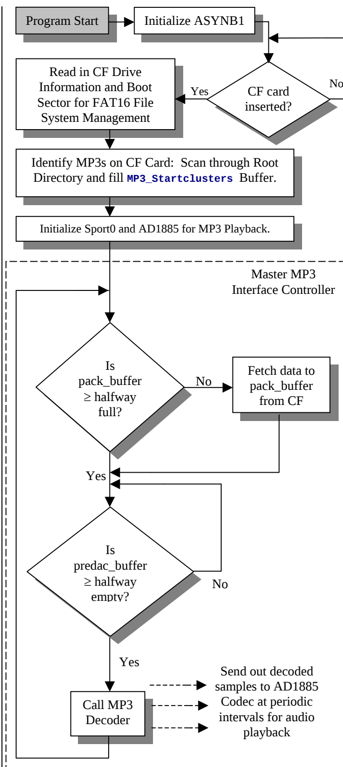
Figure 6. MP3 Software Flow
