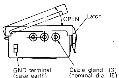
Transmitter (FQH)
