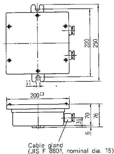
Junction box (FQGA2)
