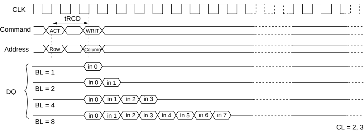
Burst write
