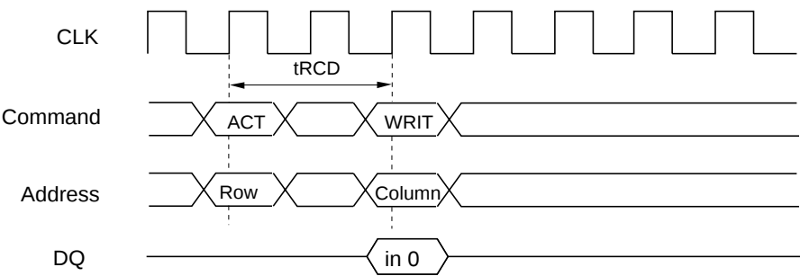
Single write
