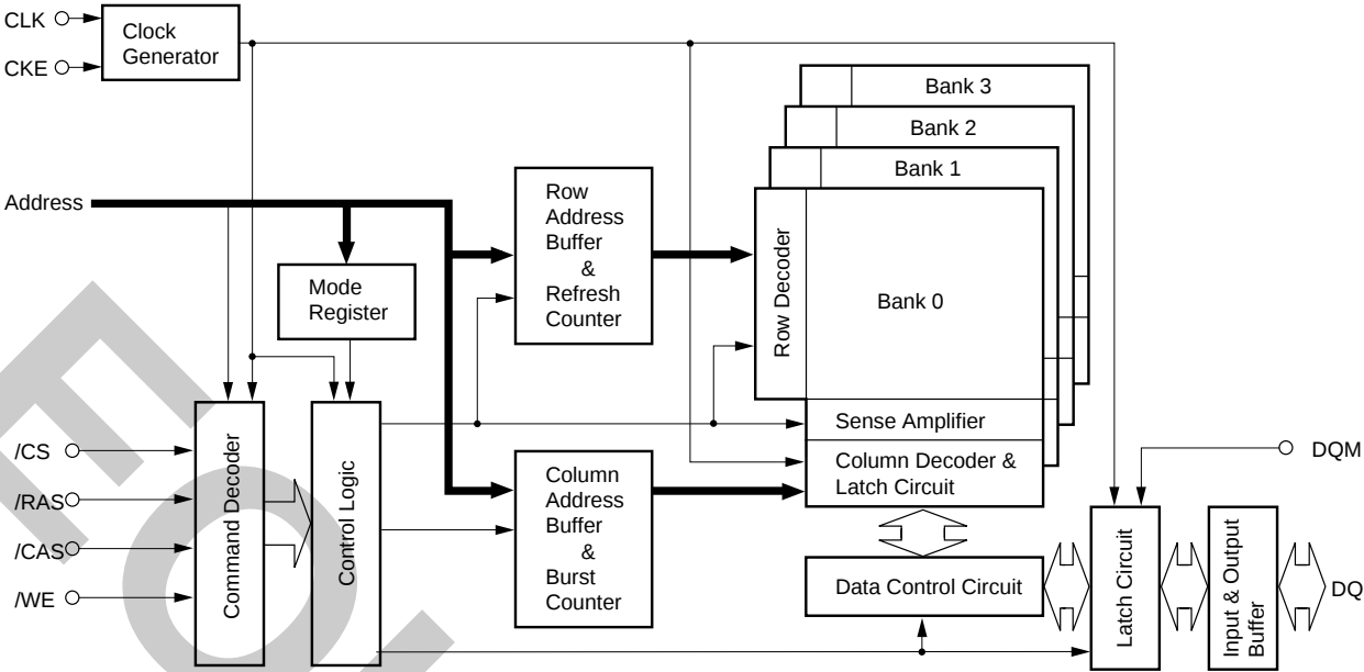
Block Diagram
