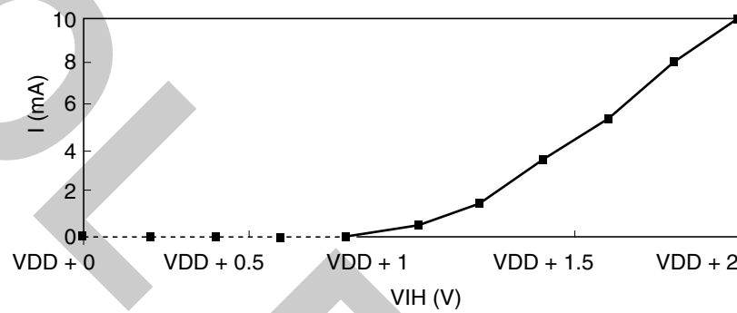
Minimum VIH Clamp Current
