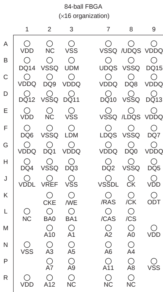
(Top view)
