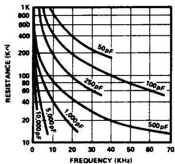
RESISTANCE vs OSCILLATOR FREQUENCY
