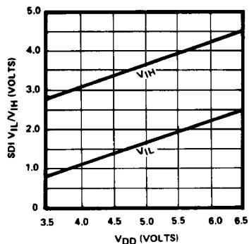
SDI INPUT V_{IL}/V_{IH} vs V_{DD}
