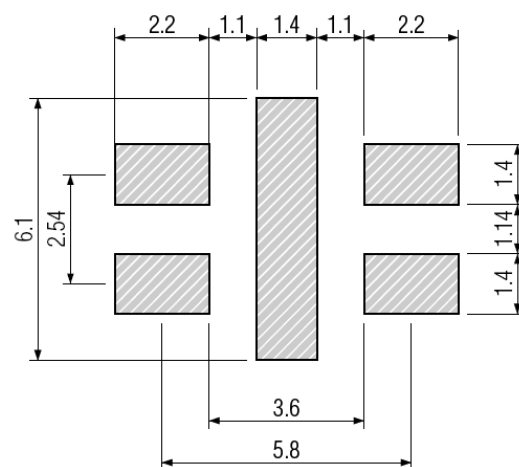
Figure 2) Land Pattern
