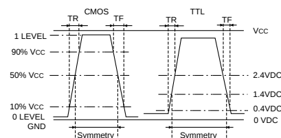
Figure 3) Output Waveform
