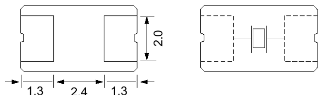
Figure 1) Top, Side, Bottom and End views
