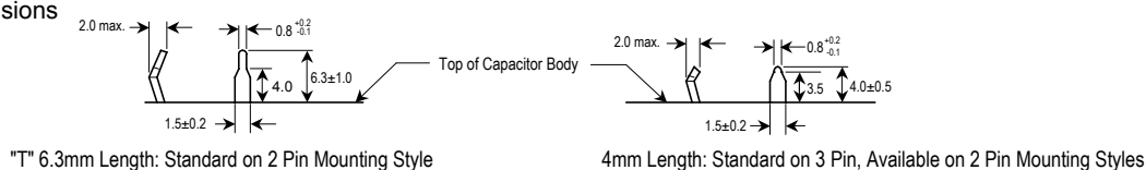
Pin Dimensions
