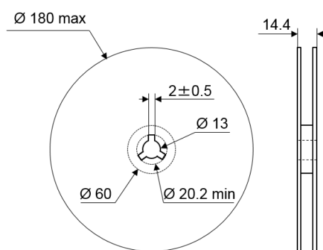
Figure 21: Reel dimensions in mm
