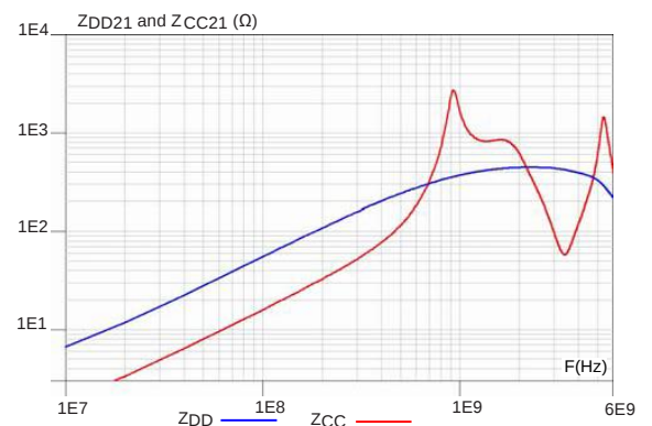
Figure 8: Differential ( Z_{DD21} ) and common mode ( Z_{CC21} ) impedance versus frequency
