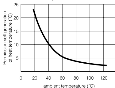
Permission self generation of heat temperature vs. ambient temperature
