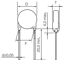
Note: Tolerance of Lead Space
