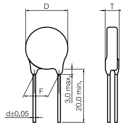
Note: Tolerance of Lead Space
