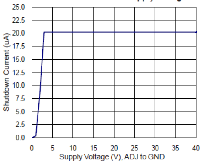
Shutdown Current vs. Supply Voltage
