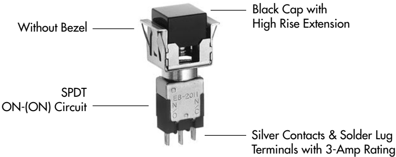
DESCRIPTION FOR TYPICAL ORDERING EXAMPLE WITHOUT BEZEL EB2011-A-J40
