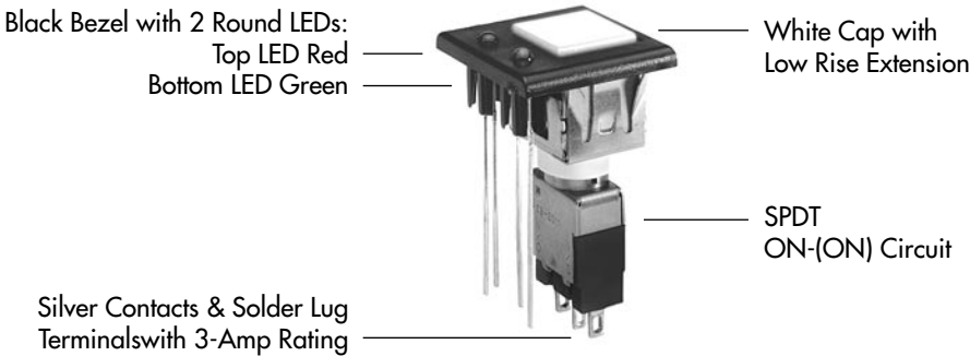
DESCRIPTION FOR TYPICAL ORDERING EXAMPLE WITH BEZEL EB2011-B-J23ACF
