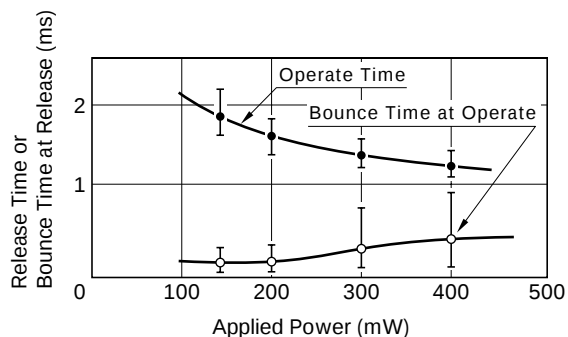
OPERATE TIME
