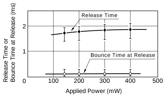
RELEASE TIME WITH DIODE
