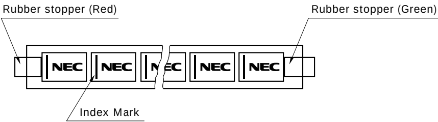
Outline of Package
