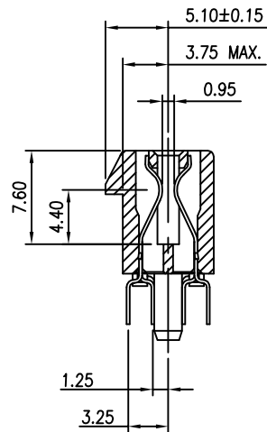
SECTION F-F
