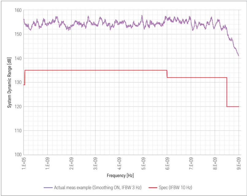
System dynamic range (specification and actual measurement data example)
