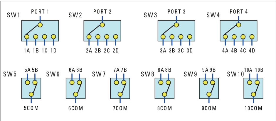
Figure 14. Switch configuration (E5092A-020)
