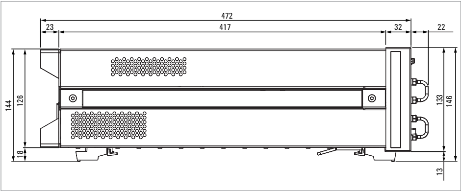
Figure 13. Dimensions (side view, with Option E5092A-020, in millimeters, nominal)
