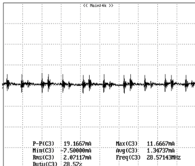
Figure 12: Input reflected ripple current, i_s , through a 12μH source inductor at nominal input voltage and rated load current (20 mA/div, 2μs/div).
