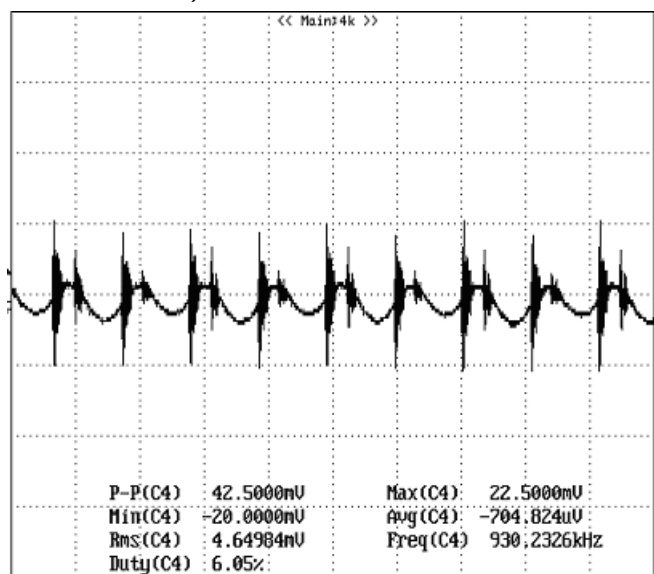
Figure 14: Output voltage ripple at nominal input voltage and rated load current ( I_o=10A ) (20 mV/div, 2μs/div) Load capacitance: 1μF ceramic capacitor and 10μF tantalum capacitor. Bandwidth: 20 MHz. Scope measurements should be made using a BNC cable (length shorter than 20 inches). Position the load between 51 mm to 76 mm (2 inches to 3 inches) from the module.
