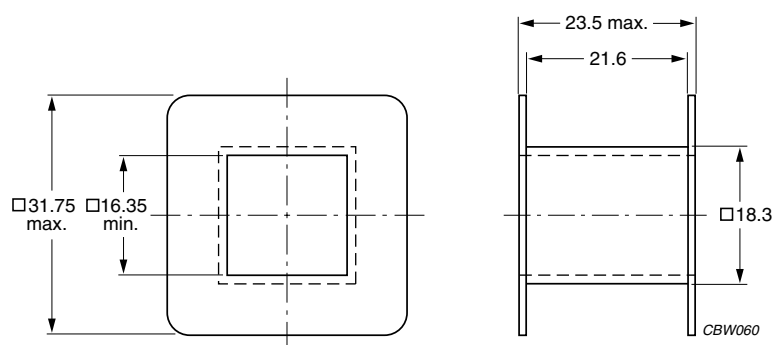
Fig.2 E47/20/16 coil former.
