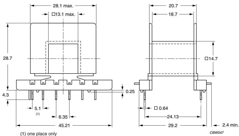
Fig.3 E41/17/12 coil former; 12-pins.
