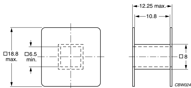
Fig.2 E25/10/6 coil former.
