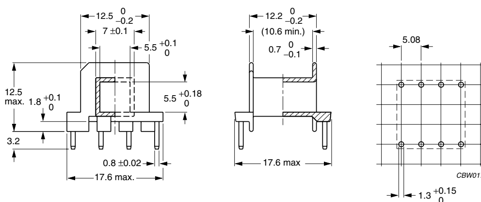
Fig.3 E20/10/5 coil former; 8-pins.
