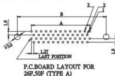
P.C. BOARD LAYOUT PATTERN
