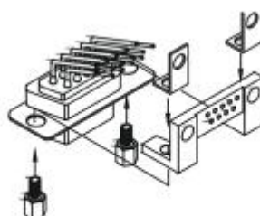
WITH BRACKET + L-SHAPE
