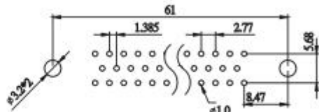
50 POSITION FEMALE/MALE
