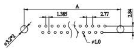
FEMALE/MALE
