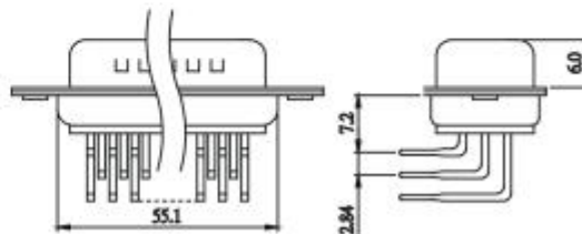
50 POSITION MALE
