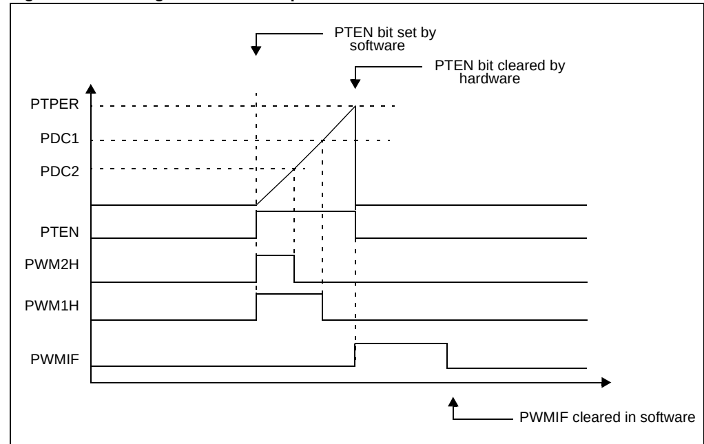
Figure 15-8: Single Event PWM Operation
