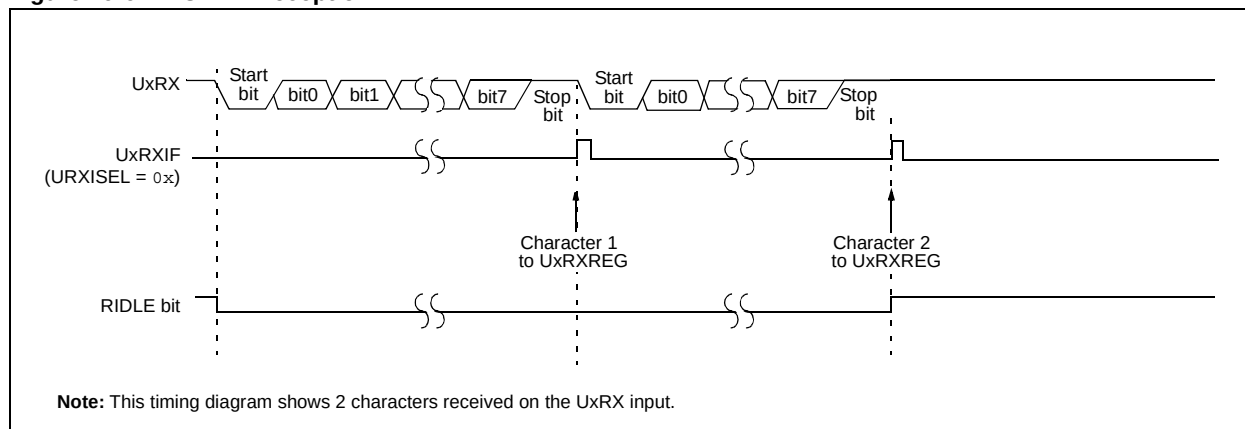
Figure 19-6: UART Reception
