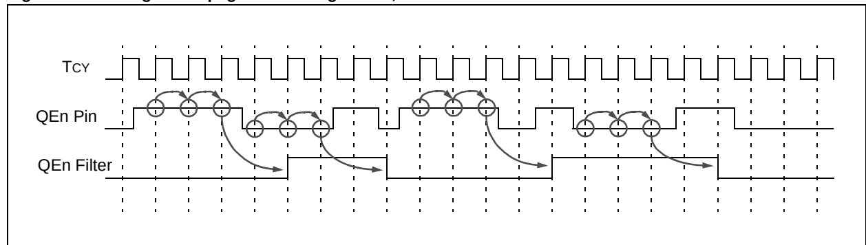
Figure 16-5: Signal Propagation Through Filter, 1:1 Filter Clock Divide
