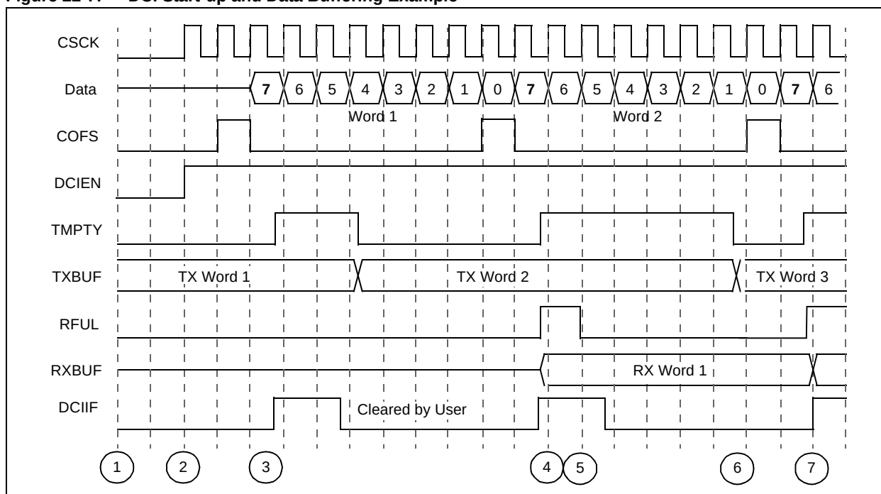
Figure 22-7: DCI Start-up and Data Buffering Example
