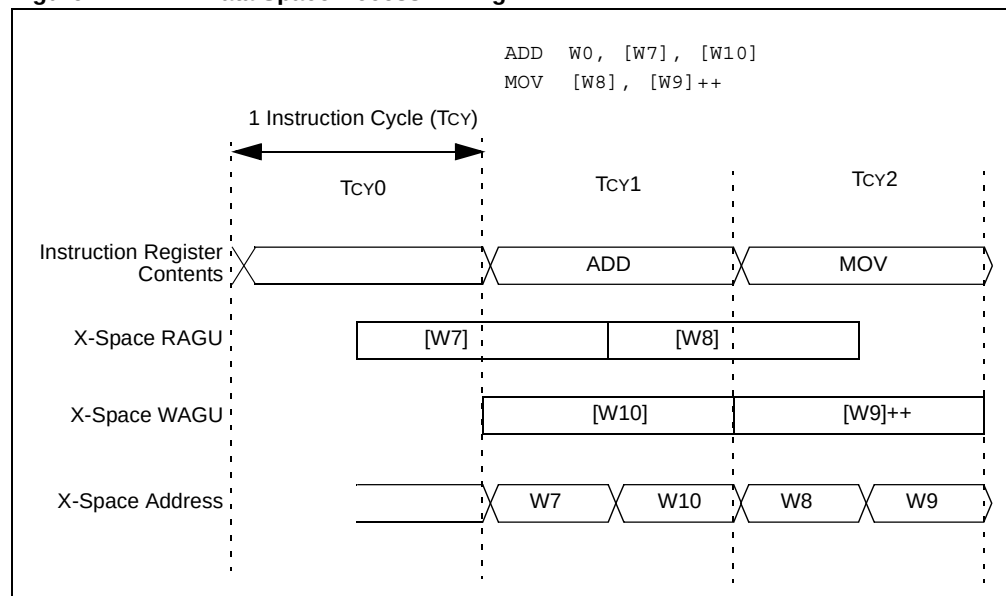
Figure 2-21: Data Space Access Timing
