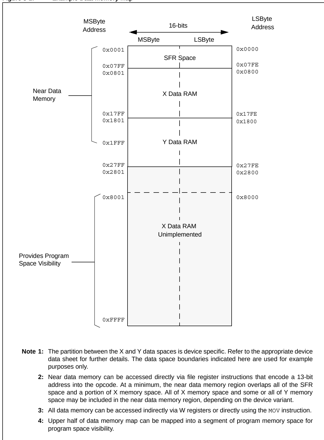
Figure 3-1: Example Data Memory Map
