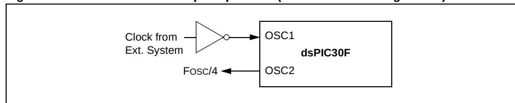
Figure 7-5: External Clock Input Operation (EC Oscillator Configuration)
