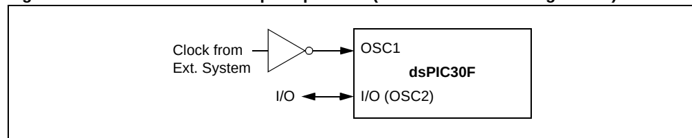
Figure 7-6: External Clock Input Operation (ECIO Oscillator Configuration)
