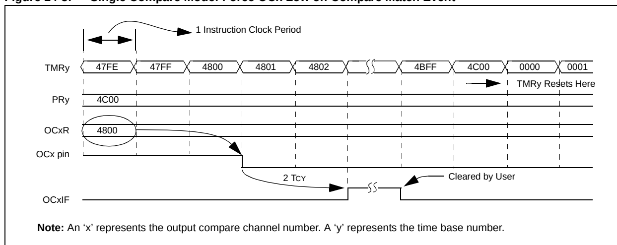
Figure 14-3: Single Compare Mode: Force OCx Low on Compare Match Event
