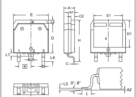
X019 TO-268 AA (D 3 PAK) Weight = 4 g
