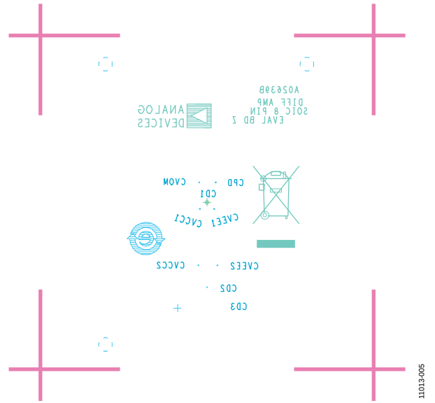
Figure 5. Bottom Silkscreen
