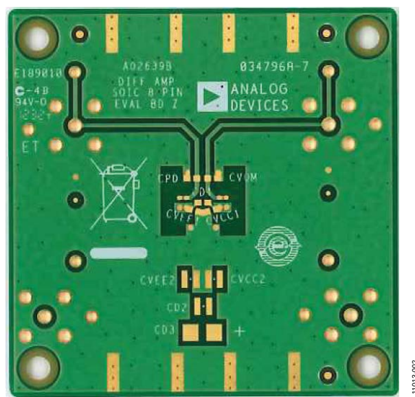
Figure 2. Evaluation Board, Circuit Side
