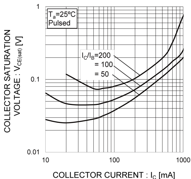
Fig.5 Collector-Emitter Saturation Voltage vs. Collector Current(I C )
