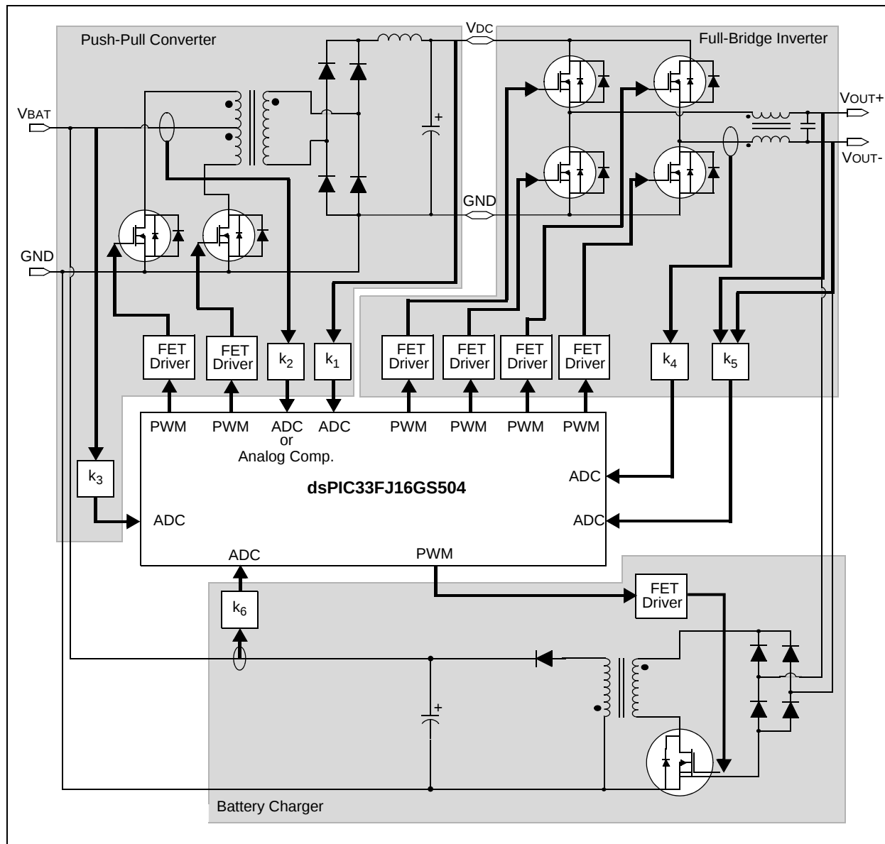
FIGURE 2-8: OFF-LINE UPS
