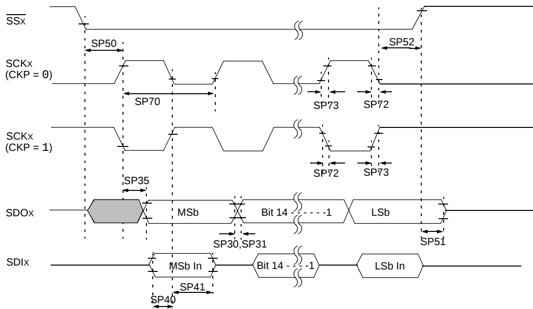
FIGURE 24-18: SPIx SLAVE MODE (FULL-DUPLEX, CKE = 0, CKP = 0, SMP = 0) TIMING CHARACTERISTICS
