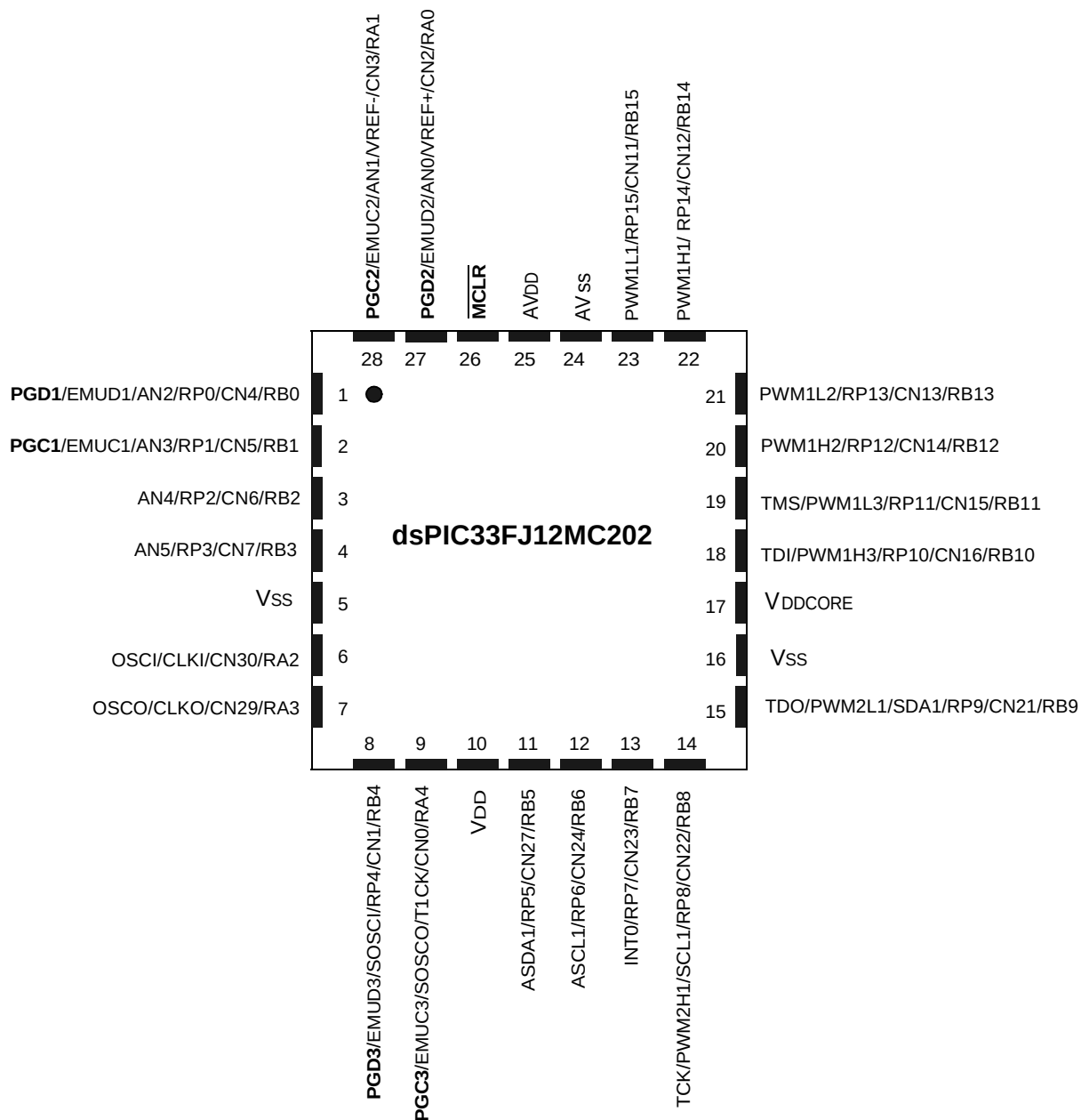
28-Pin QFN 6*6mm
