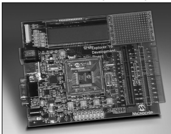
FIGURE 13-2: EXPLORER 16 DEVELOPMENT BOARD
