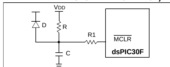
FIGURE 18-11: EXTERNAL POWER-ON RESET CIRCUIT (FOR SLOW V_{DD} POWER-UP)
