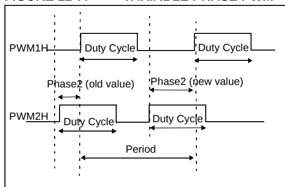
FIGURE 12-7: VARIABLE PHASE PWM
